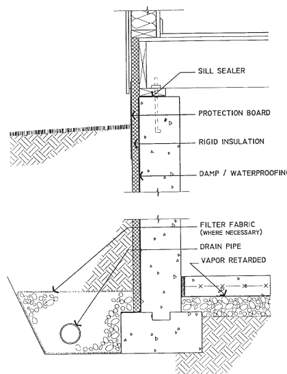
CONCRETE BASEMENT WALL WITH EXTERIOR INSULATION
