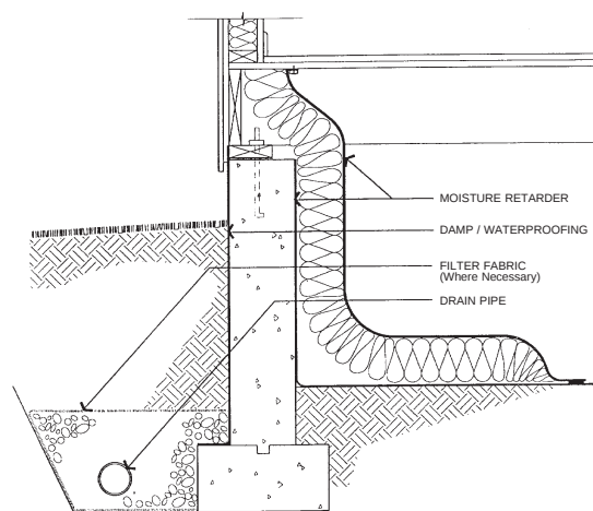
FIGURE 5, 6. CONCRETE CRAWL SPACE WALL WITH INTERIOR INSULATION
