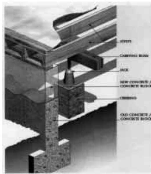
FIGURE 5. JACKING A WALL WITH PERPENDICULAR JOISTS
