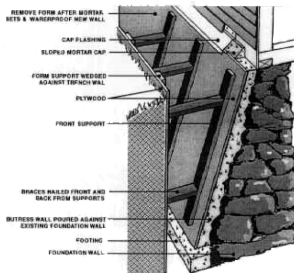
BUTTRESSING STONE FOUNDATION WALL
