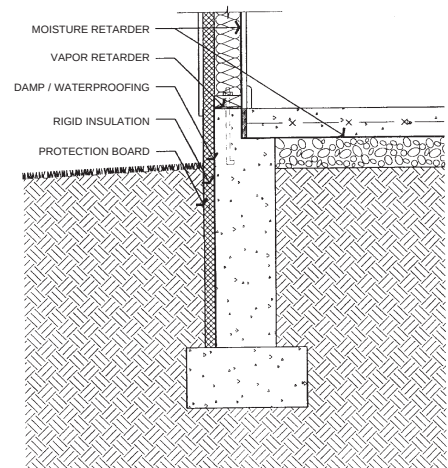
SLAB-ON-GRADE WITH CONCRETE STEM BEAM
